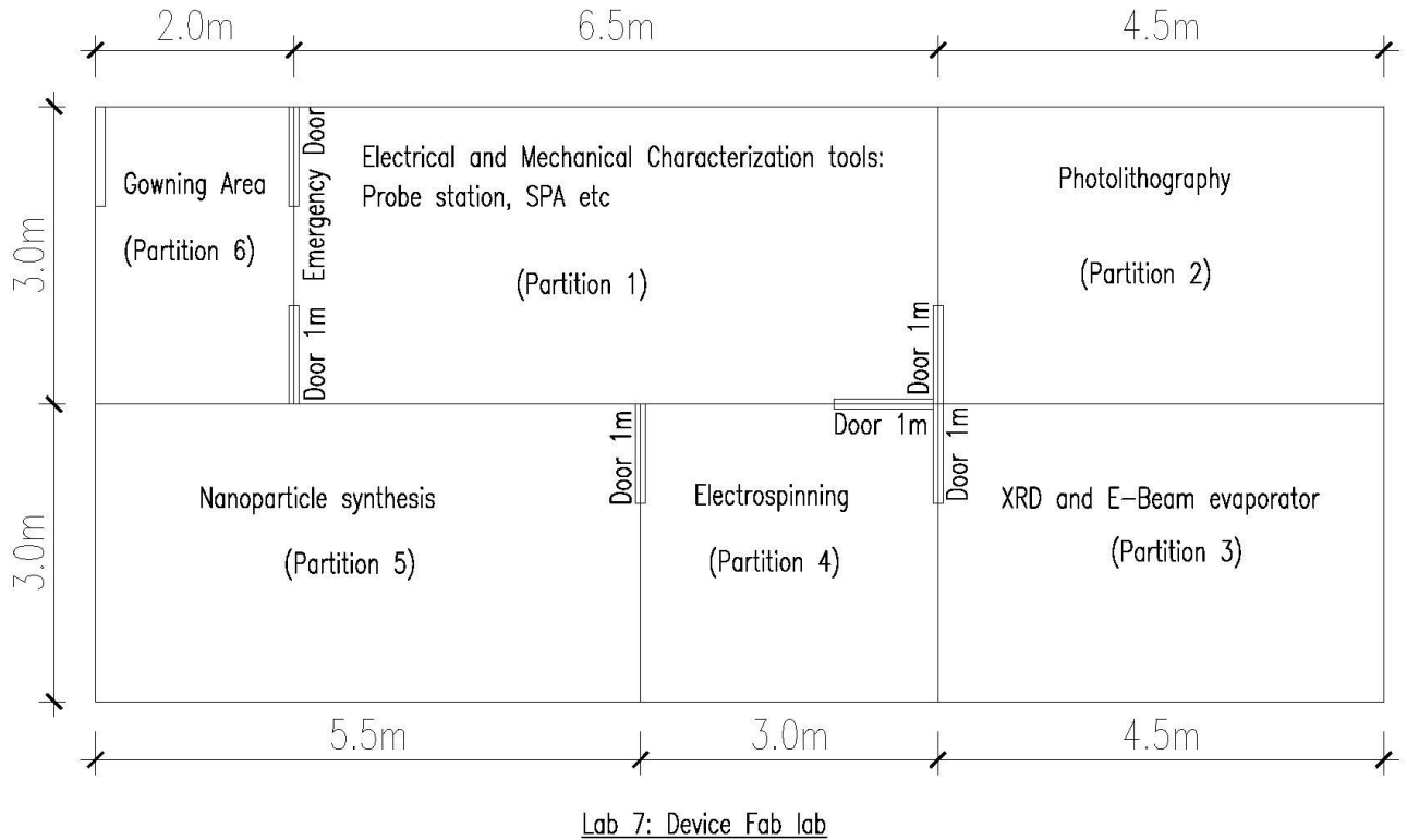
Figure 1: Schematic layout of clean room (Lab 7)
